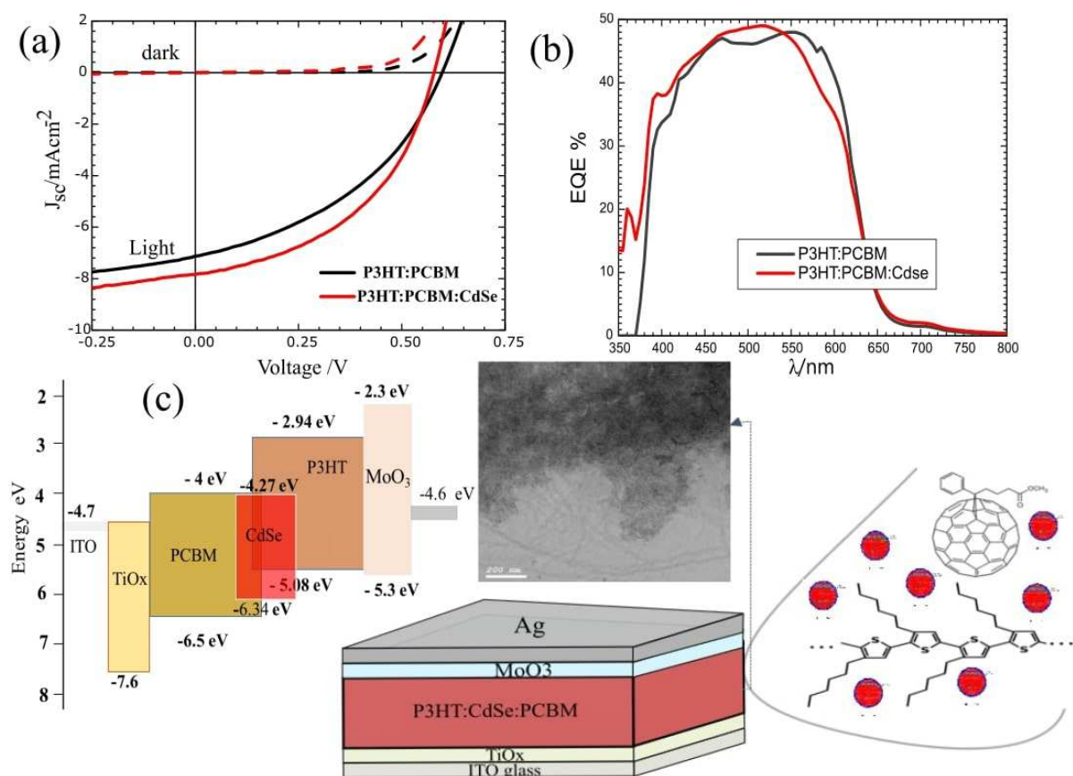
Fig. 4. (a) The J-V characteristics of ITO/TiO x /P3HT:PC60BM:CdSe/MoO 3 /Ag (red) and ITO/TiO x /P3HT:PC60BM/MoO 3 /Ag (Black) Low temperature studies of the photoluminescence from colloidal CdSe nanocrystals prepared by the hot injection method in liquid paraffin shown in dark and under AM1.5 illuminations. (b) Spectral EQE characteristics of both devices. (C) Representation of the cell structure and the corresponding band diagram. It also shows a cartoon drawing for the active layer with CdSe QDs. (d) TEM image for P3HT:PCBM:CdSe QDs.
