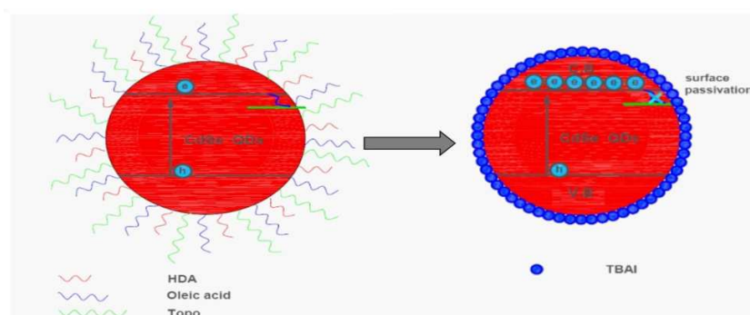
Fig.1. Cartoon drawing for the as-synthesized CdSe QDs and the Iodide treated dots
