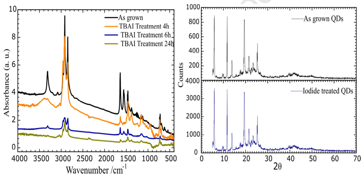
Fig. 3. (a) The Fourier transform infrared spectroscopy (FTIR) shows the changes in the vibronic modes upon treatment of the CdSe nanocrystal with the iodide ligand at a different time interval of 4h, 6h, and 24 h indicate the depletion of the TOPO/HDA/OA and the successive substitution by iodide ligand. (b) The X-ray diffraction pattern of the as-grown CdSe quantum dots and iodide treated dots.
